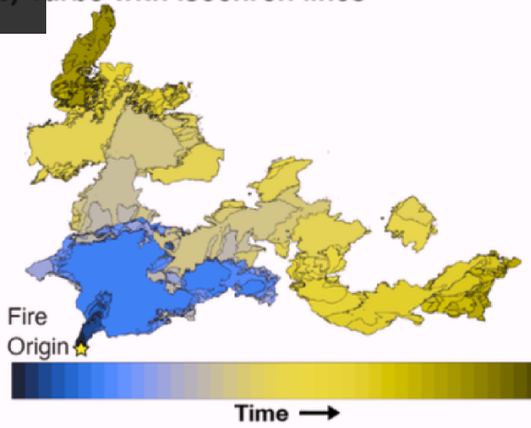
d) Batlow with isochron lines
