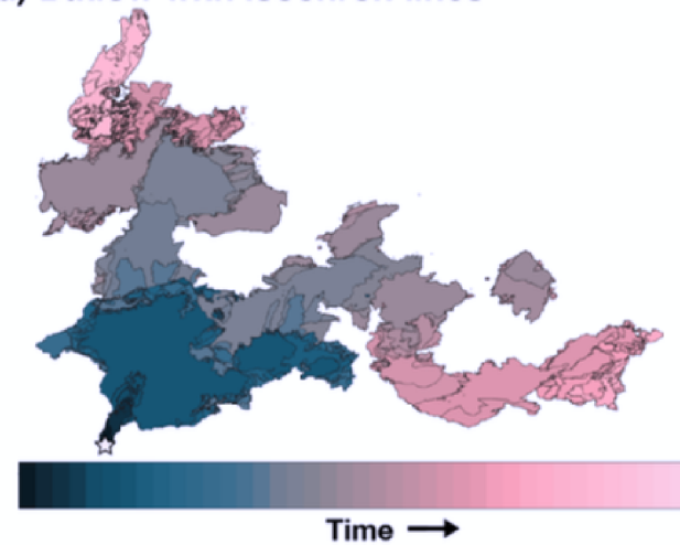
f) Reversed Managua with isochron lines
