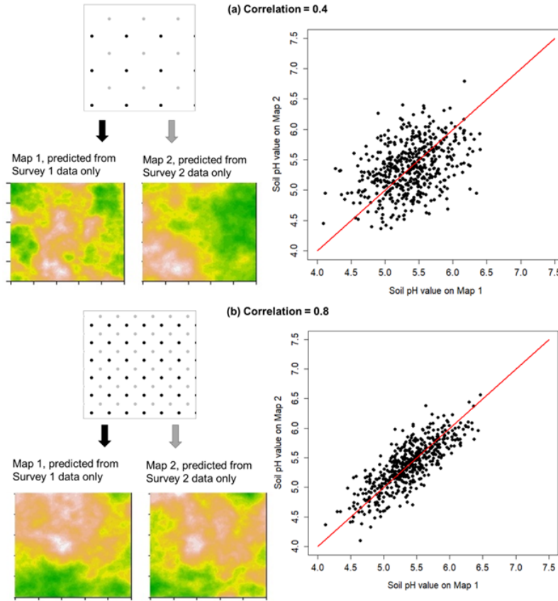
Figure 1. The pair-illustration of the offset correlation in two hypothetical maps-cases where this takes values of pH-value-0.4 (a) and corresponding scatter-plot for 0.8 (b). In each case the illustrated subset of grid points is of the same dimensions, so the grid is denser in (b) than (a). In each case a hypothetical data set 1 (black grid points) and set 2 (grey points) is collected from grids of shared spacing but offset north-south and east-west by half the grid spacing. The offset correlation 0.4 is the correlation of the predictions of the soil properties made at common sites from the two grids. In practice this is calculated theoretically from the variogram and a proposed grid spacing to assess the sensitivity of the original map to variation in the position of the grid origin.
