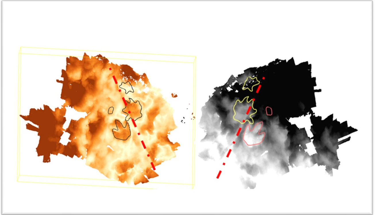
420 Figure 7 Shows the same images shown in figure 6 but the natural color of the images has been replaced by colors that vary with depth. The red dashed line shows the location of a fracture imaged in the model. The red dashed line shows the location of a fracture in the rocks and the footprints are outlined in this image.
