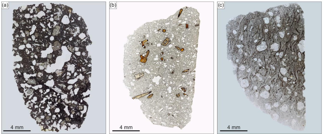
625 Figure 1: Thin section samples selected for use in the prototype learning resource. a) Basalt, b) Andesite, c) Rhyolite
