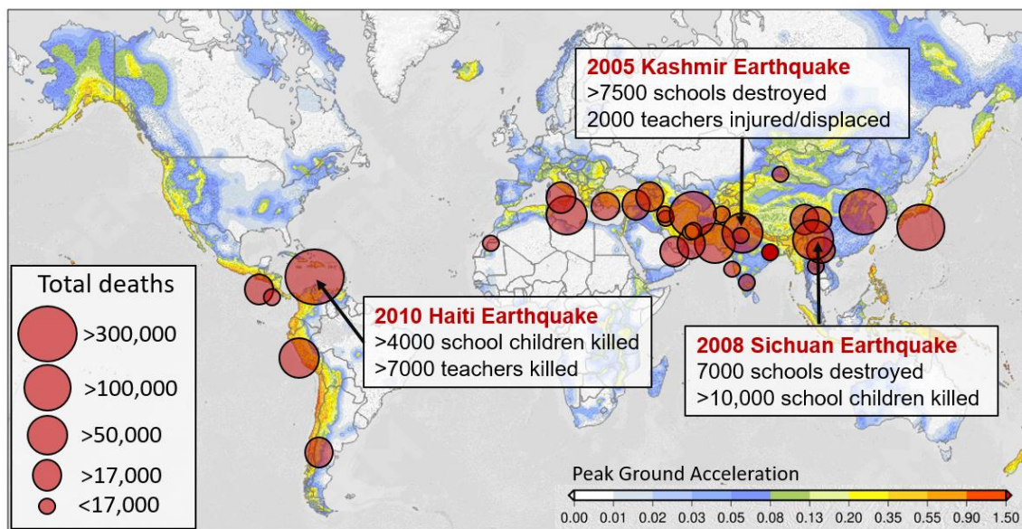
580 Figure 1. Significant earthquakes from NOAA database superimposed on the Global Seismic Hazard map of Pegani et al. (2018). Impact 585 details of recent earthquakes discussed in text are shown in white boxes.
