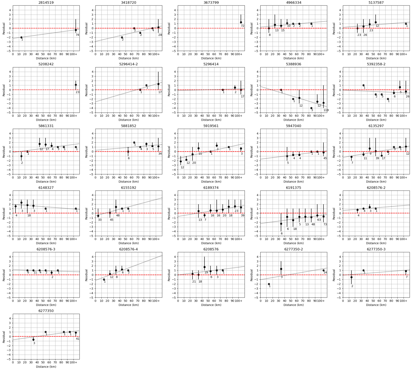
Figure 7. Residuals of predicted and observed MCSs. Red dashed line represents the baseline. Black circles are the residual of weighted average of the bin. Vertical black lines are the residuals from predicted MCSs and minimum and maximum MCSs that are observed in the bin. Black dotted line is the fitted line to the residual of weighted averages. Number of data points inside bins are provided beneath each bin point with data (created using Matplotlib library of Python).
