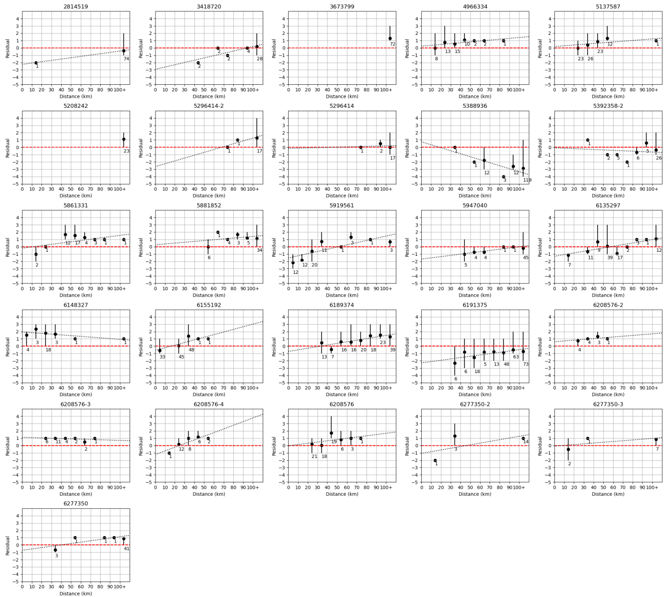
Figure 7. Residuals of predicted and observed MCSs-MSCs . Red dashed line represents the baseline. Black circles are the residual of weighted average of the bin. Vertical black lines are the residuals from predicted MCSs-MSCs and minimum and maximum MCSs-MSCs that are observed in the bin. Black dotted line is the fitted line to the residual of weighted averages. Number of data points inside bins are provided beneath each bin point with data (created using Matplotlib library of Python).
