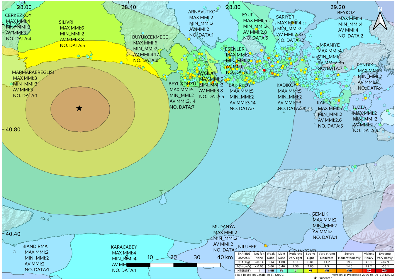
Figure 4. Intensity map of 26th-26 September 2019 Istanbul earthquake with labelled entries. Entries are plotted to district level polygons. Felt reports of the earthquake submitted to EMSC on top of the labelled entries (created using QGIS).
