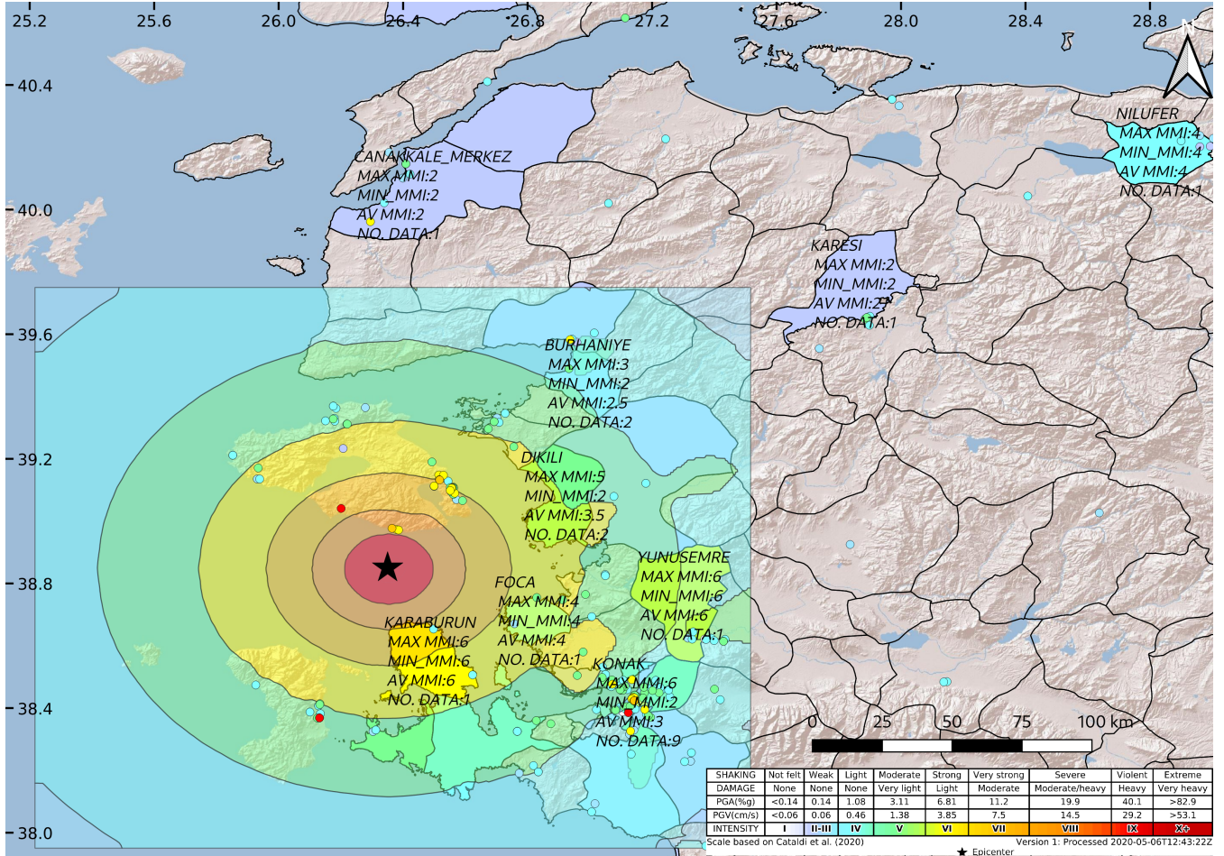
Figure 1. Intensity map of 12th 12 June 2017 Lesbos earthquake with labelled entries. Entries are plotted to district level polygons since the exact location of data providers are unknown. Felt reports of the earthquake submitted to EMSC on top of the labelled entries (created using QGIS).
