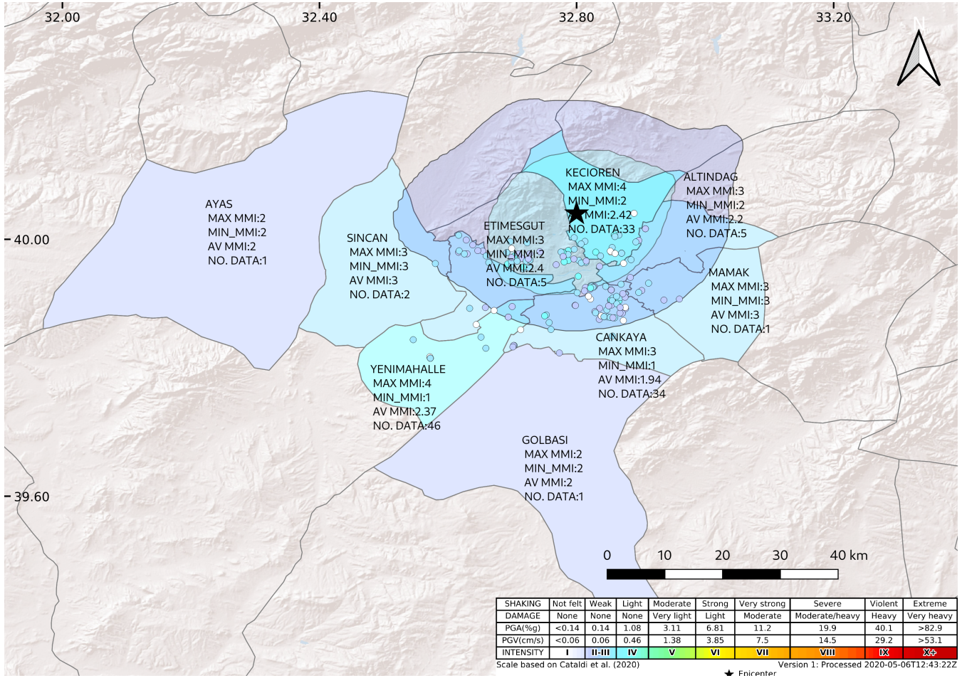
Figure 3. Intensity map of 25th-25 August 2019 Ankara earthquake with labelled entries. Entries are plotted to district level polygons. Felt reports of the earthquake submitted to EMSC on top of the labelled entries (created using QGIS).
