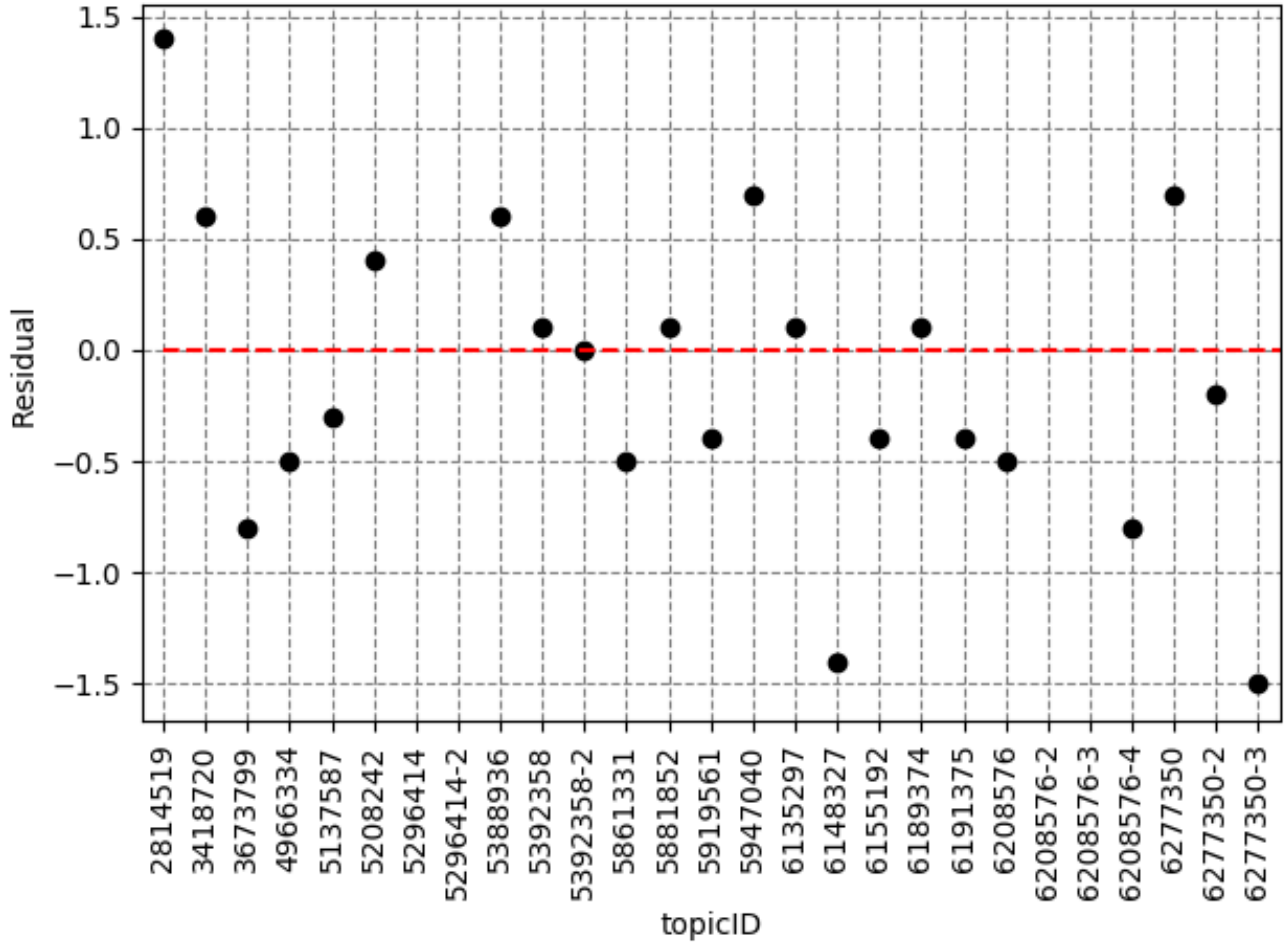
Figure 6. Residuals of measured magnitudes of the earthquakes (Table 1) with average magnitude guesses from users. Earthquakes without any guesses are blank ( created using Matplotlib library of Python ).
