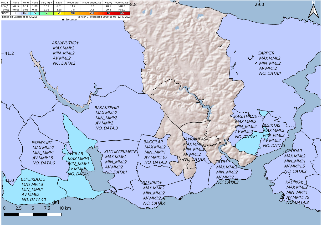
Figure 2. Intensity map of 12th-13 June 2017 Lesbos earthquake with labelled entries in West side of Istanbul. Entries are plotted to district level polygons (created using QGIS).
