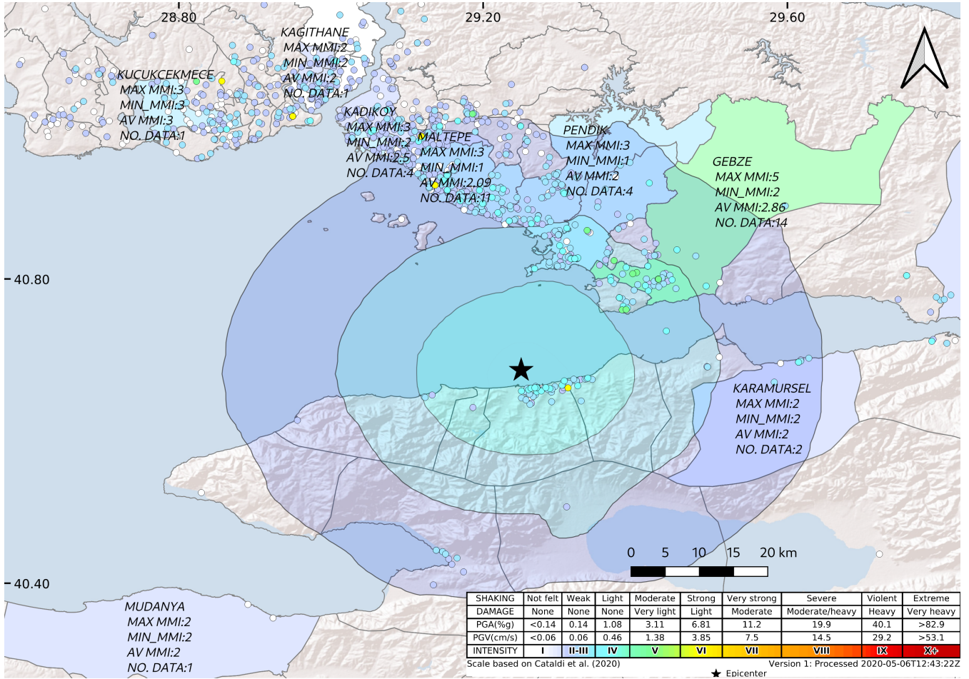
Figure 5. Intensity map of 10th October 2019 Yalova earthquake with labelled entries. Entries are plotted to district level polygons. Felt reports of the earthquake submitted to EMSC on top of the labelled entries (created using QGIS).
