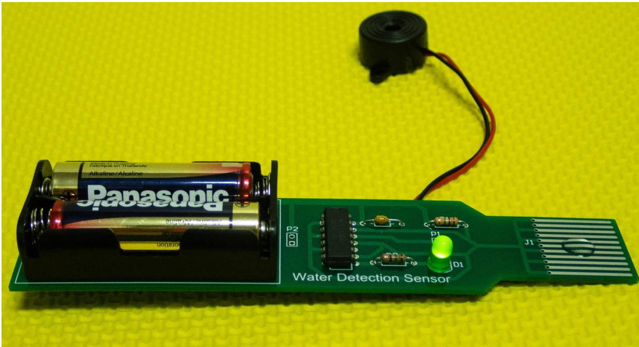
1055 Fig. 7. Water detection PCB. A droplet of water turns on the light-emitting diode (LED) and an attached piezoelectric buzzer to provide visual and audible feedback.
