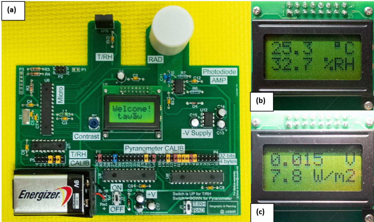
1075 Fig. 8. (a) Hybrid temperature, relative humidity (RH) and solar radiation sensor. (b) LCD display showing calibrated 1080 calibrated temperature and relative humidity (RH) readout. (c) LCD display showing calibrated voltage output and radiation flux in \text{W m}^{-2} . Calibration coefficients are set using removable plastic jumpers and the position of each calibration header is indicated by “CALIB” marked on the PCB silkscreen. The “T/RH” marking indicates the position of the temperature and RH sensor, whereas the “RAD” marking indicates the position of the pyranometer sensor comprised of a photodiode and an op-amp. The photodiode is covered with a piece of plastic pipe and a circular Teflon diffuser. This ensures that the photodiode has a cosine response to obtain a hemispherical measurement. Other markings indicate the positions of various PCB sub-systems, including a switch for setting the mode of circuit operation and a contrast adjustment potentiometer.
