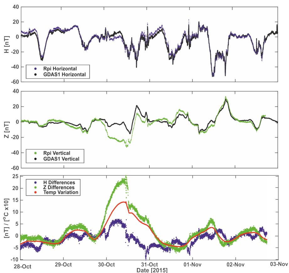
Figure 3. Comparison of the magnetic field variation between the Raspberry Pi magnetometer and Eskdalemuir GDAS1 system from 28-Oct-2015 to 03-Nov-2015. Upper panel: Horizontal component variation; Middle panel: Vertical component variation; Lower panel: Difference between the two systems with the temperature variation (x10) also plotted.
