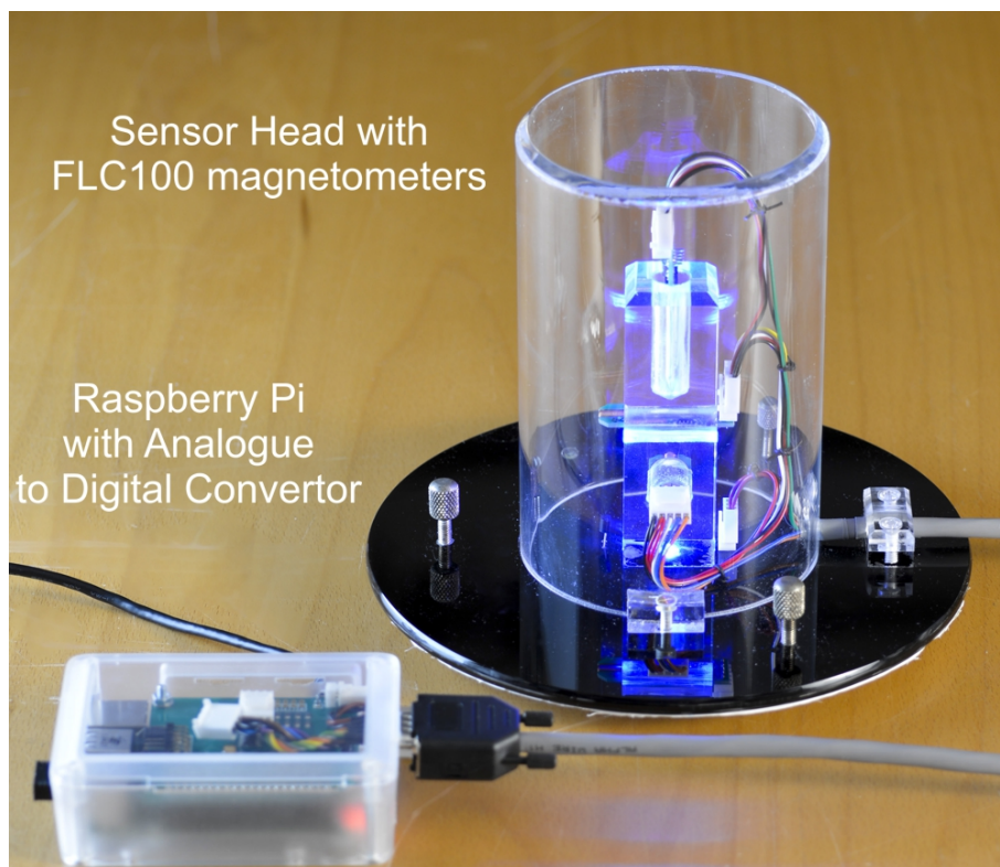
Figure 1. Raspberry Pi magnetometer system. The sensor head is approximately 15 cm high.
