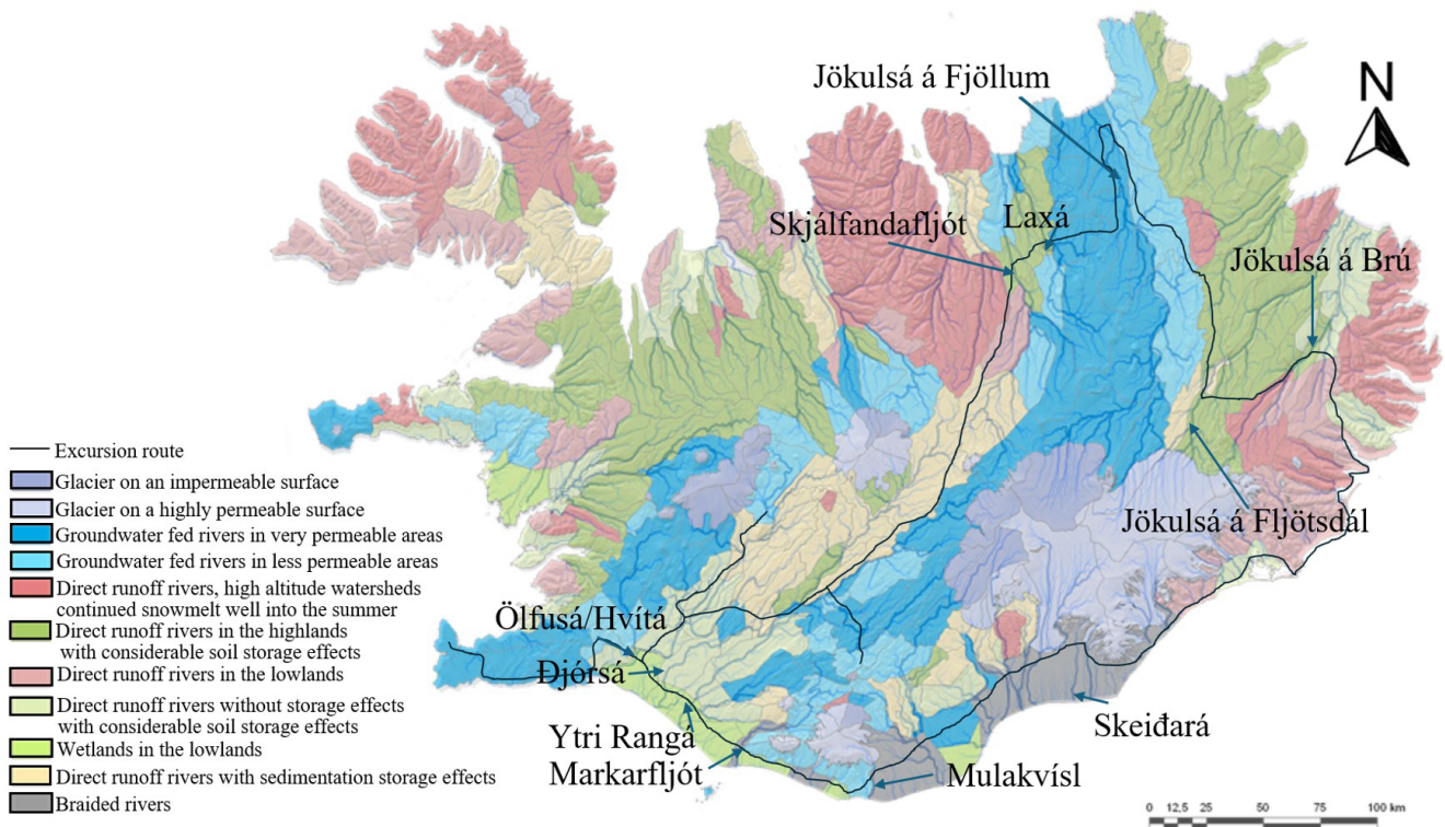
Figure 2. Hydrological classification and major rivers (modified from Jóhannesson et al., 2007 and SDI Iceland, 2026). Names indicate major rivers in Iceland which are visited and discussed during the excursion.
