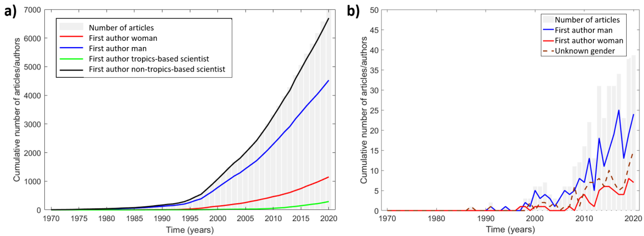
Figure 1. Cumulative number of articles published in the cloud physics community during the last 50 years for (a) all geographic locations and (b) tropics-based authors. In panel (a) the red, blue, green, and black lines indicate if the first author is woman, man, a tropics-based scientist, or a non-tropics-based scientist, respectively. In panel (b) the blue, red, and brown lines indicate if the first author is man, woman, and with unknown gender, respectively.
