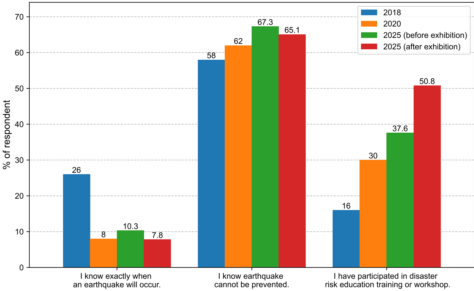
Earthquake-related knowledge
