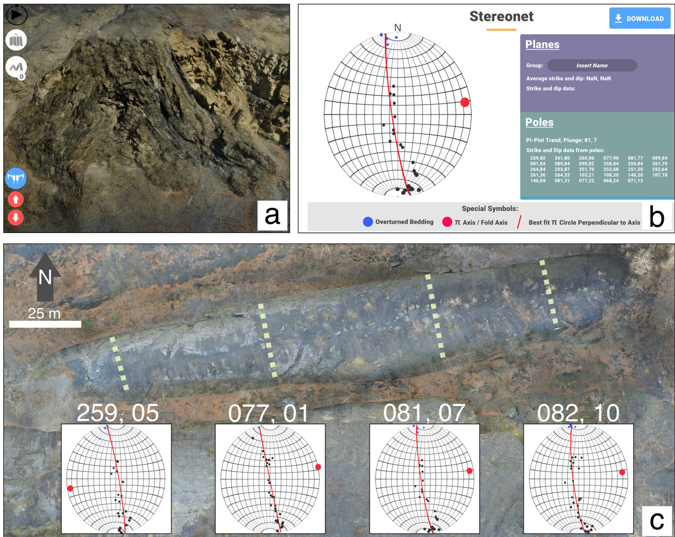
Figure 2. Examples of exercises and data. (a) An anticline (and, often, the adjacent syncline) exposed in profile in the eastern wall of the strip mine was a common feature that the students selected for description. The field of view is 55 m wide. (b) A screenshot of data from a scan line used to determine the trend and plunge of the fold axis of the Whaleback in the central eastern quarter. The fold axis orientation, generated from an automatic pi plot feature, is exaggerated as a red circle; the data for each measurement are printed on the right. (c) Students annotated an orthophoto of the Whaleback with stereonet data to investigate variations in the fold axis and best characterize the fold geometry. Each stereonet is associated with a student-made scan line (shown as a dashed line) on a section of the fold, with the trend and plunge values of the calculated fold axis printed above.
