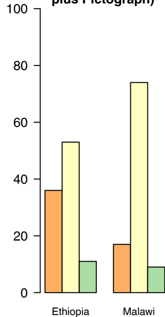
(e) Poster 4b (Raw probability plus Pictograph)
