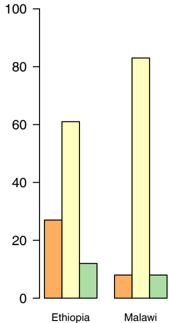
(b) Poster 2 (IPCC Verbal Scale)
