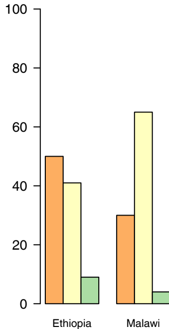
(c) Poster 3 (Kriging Variance)
