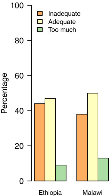
(a) Poster 1 (Prediction Interval)
